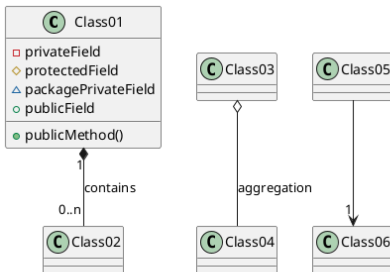
Figure 2. Class diagram
