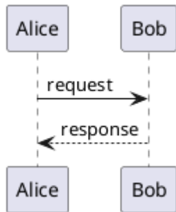
Figure 1. Sequence diagram
