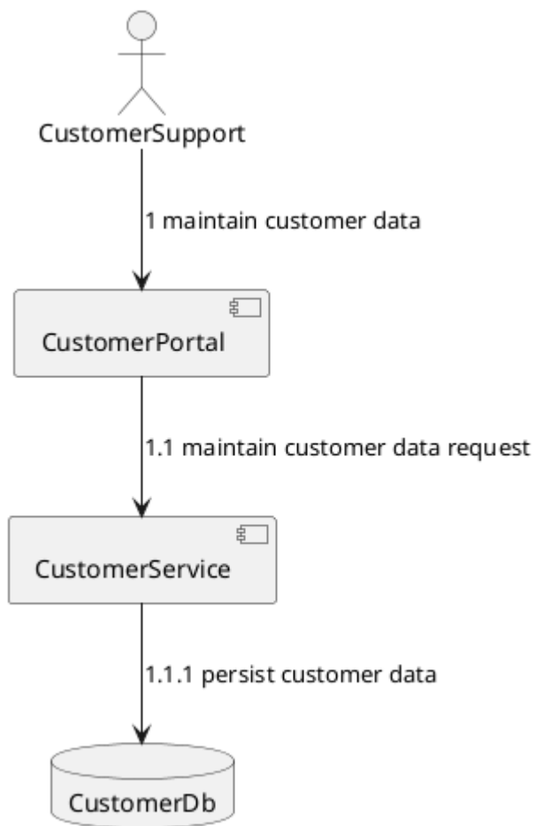
Figure 3. Component diagram
